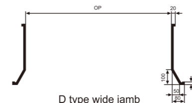
D type wide jamb
