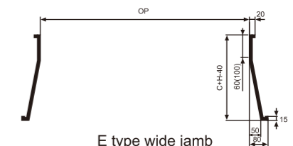
E type wide jamb
